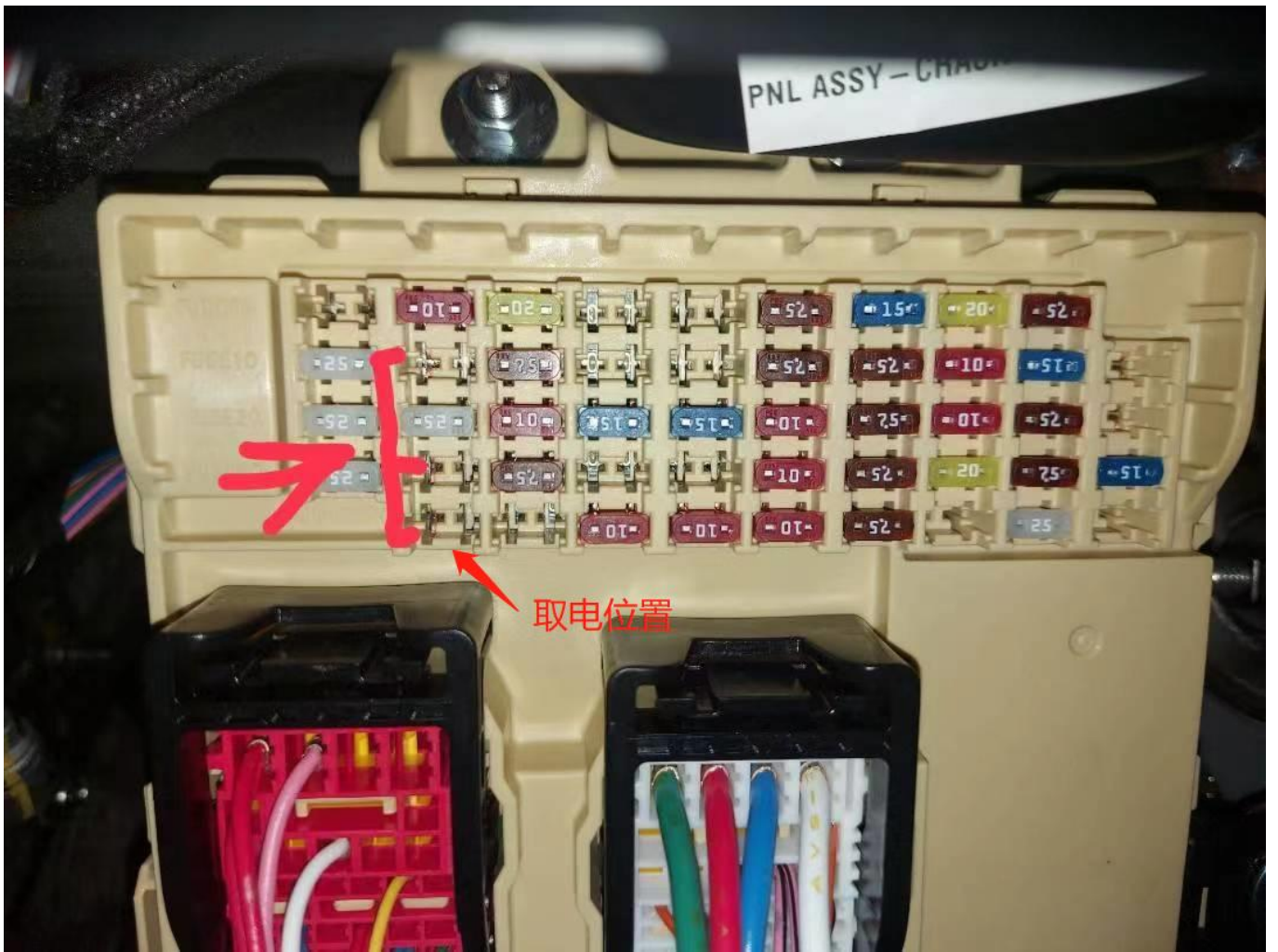
8.如下图接中控线Connect the central control line as shown below
