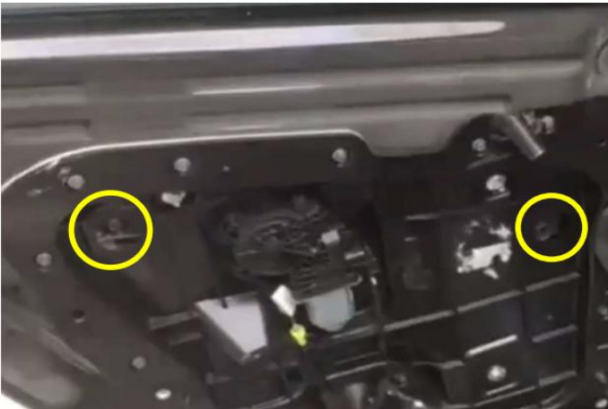
(3). 拿出标示处胶条和胶塞把玻璃螺丝对上孔位 Take out the rubber strip and rubber plug at the marking point and align the glass screw with the hole
