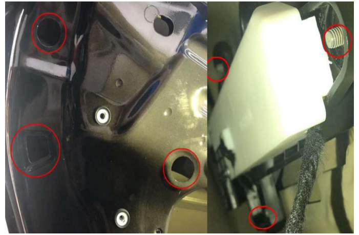
(6).取出上图三颗螺丝，拆下原车把手 Take out the three screws in the picture above and remove the original handlebar
