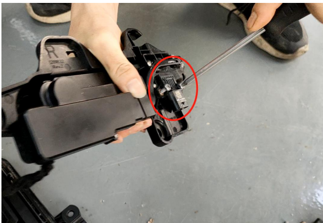
(7).将原车上的信号器拆装到相对应的电动把手上，用原车螺丝固定 Disassemble the signal on the original vehicle to the corresponding electric handle and fix it with the original vehicle screw
