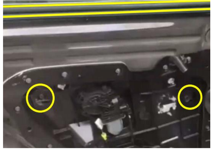
(6).拿出标示处胶条和胶塞把两圆圈内玻璃螺丝拧出就可以直接把玻璃拿出来了 Take out the rubber strip and rubber plug at the mark and unscrew the glass screws inside the two circles to take out the glass directly
