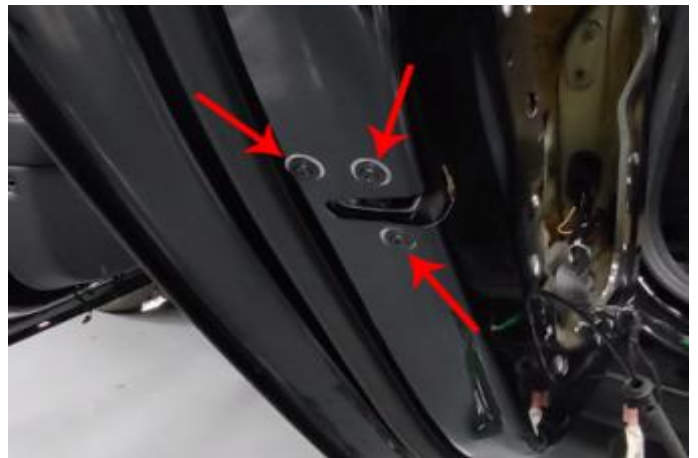
(8) .取出上图三颗螺丝，拆下原车锁 Take out the three screws shown above and remove the original lock
