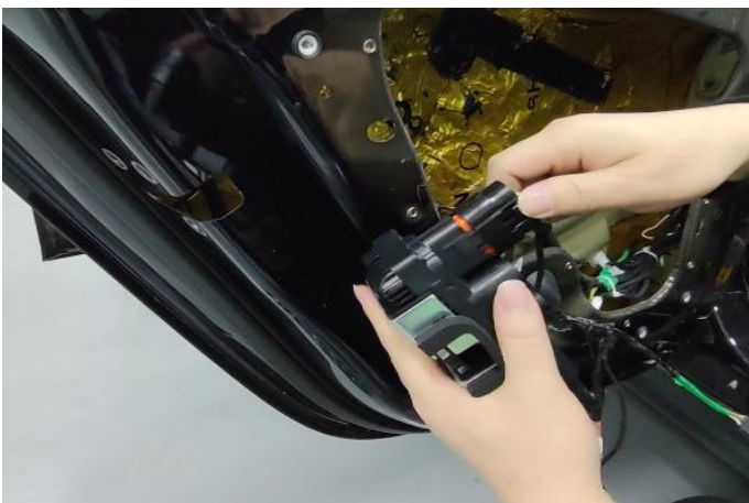
(9) .将原车插头和我司智能一体锁连接 Connect the plug of the original car with our company intelligent integrated lock
