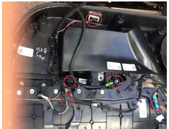
(4) .把与盖板相连的插线拔下 拿下盖板 Remove the plug wire connected to the cover plate and remove the cover plate
