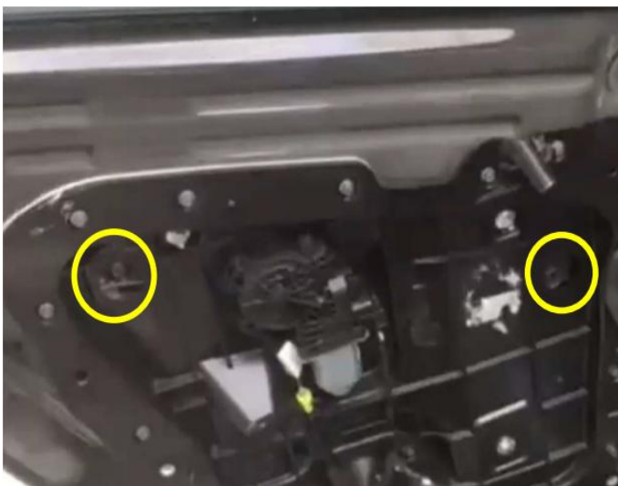
(3) .拿出标示处胶条和胶塞把玻璃螺丝对上孔位 Take out the rubber strip and rubber plug at the marking point and align the glass screw with the hole
