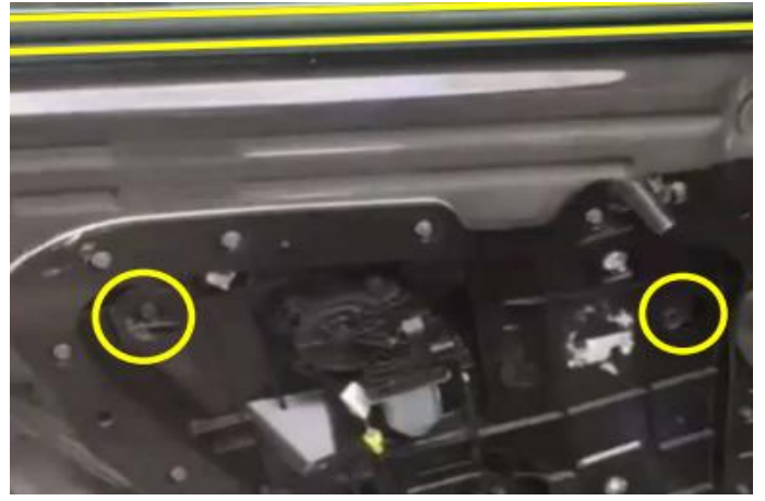
(6).拿出标示处胶条和胶塞把两圆圈内玻璃螺丝拧出就可以直接把玻璃拿出来了 Take out the rubber strip and rubber plug at the mark and unscrew the glass screws inside the two circles to take out the glass directly
