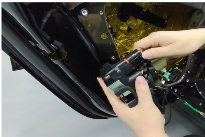
(7) .将原车插头和我司智能一体锁连接 Connect the plug of the original car with our company intelligent integrated lock
